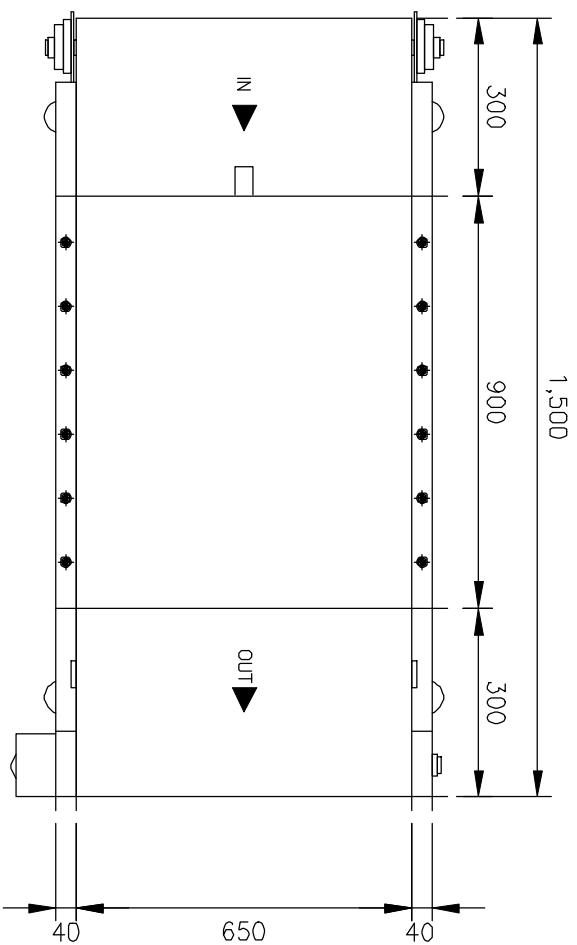
TOP VIEW SCALE NTS
