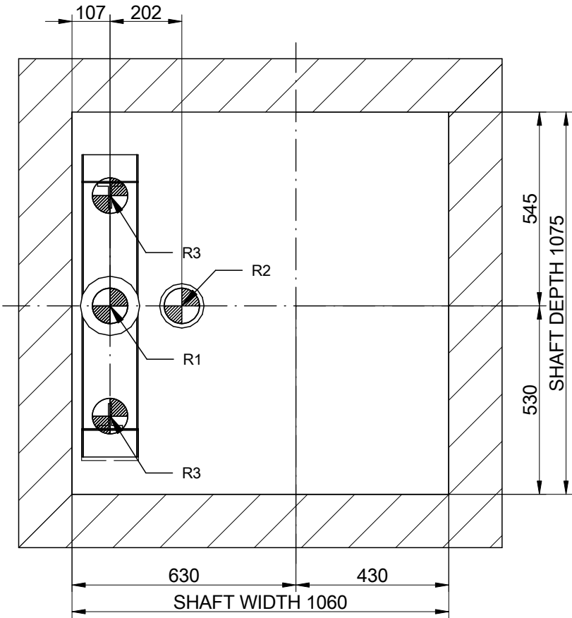
PIT LAYOUT SCALE(*): 1:15
