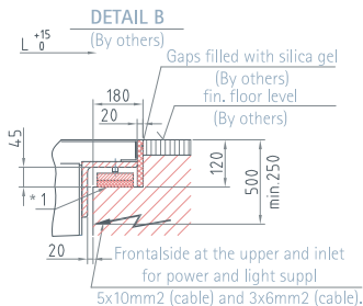
VERTICAL/INCLINED BALUSTRADE
